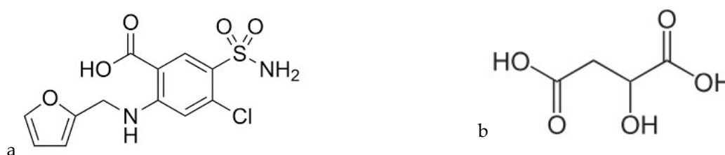
Figure 3. Molecular structure of (a) furosemide [24] and (b) malic acid [25].
