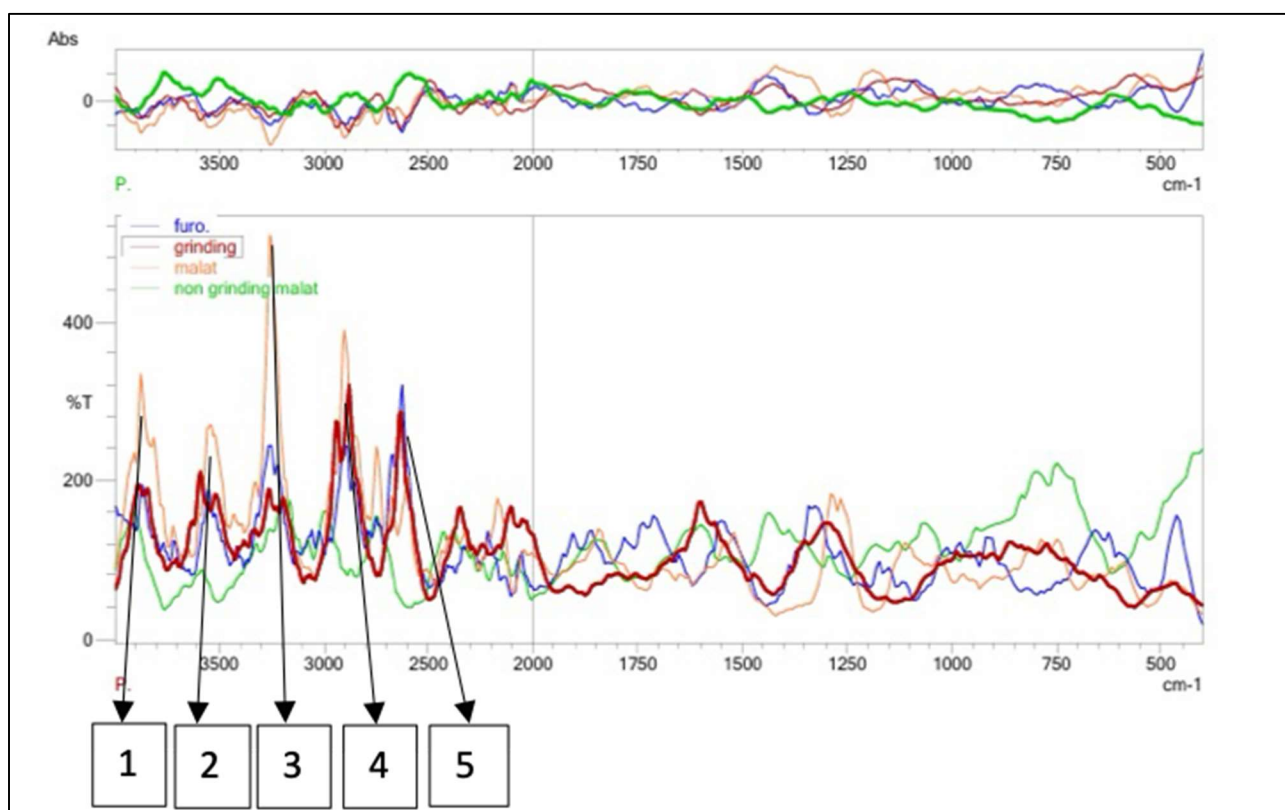
Figure 2. FTIR overlay spectrum of furosemide-malic acid and optimal cocrystal formula.
