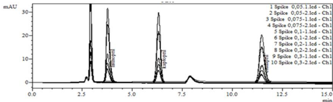
Figure 3. Chromatograms of various concentration of captopril, lisinopril and enalapril in the sample matrix.
