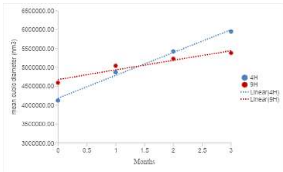
Figure 3. Ostwald ripening rate of 4H and 9H.
