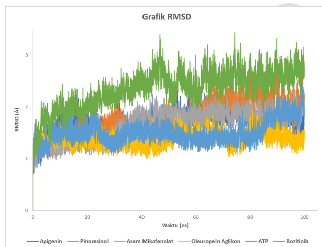
Figure 5. RMSD plots for the compounds apigenin, pinolesinol, mycophenolic acid, oleuropein aglycone, the natural ligand (ATP), and the comparator drug (bozitinib).
