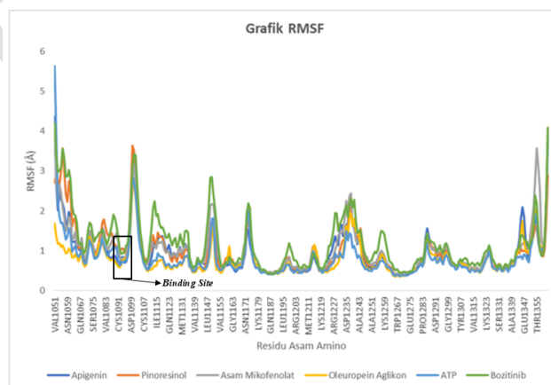
Figure 6. RMSF plots for the compounds apigenin, pinolesinol, mycophenolic acid, oleuropein aglycone, the natural ligand (ATP), and the comparator drug (bozitinib).
