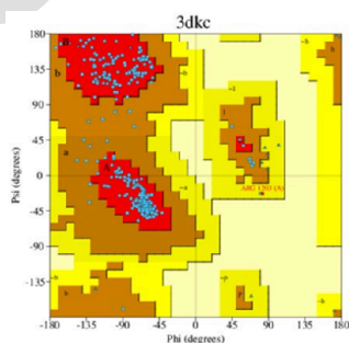
Ramachandran Plot statistics
